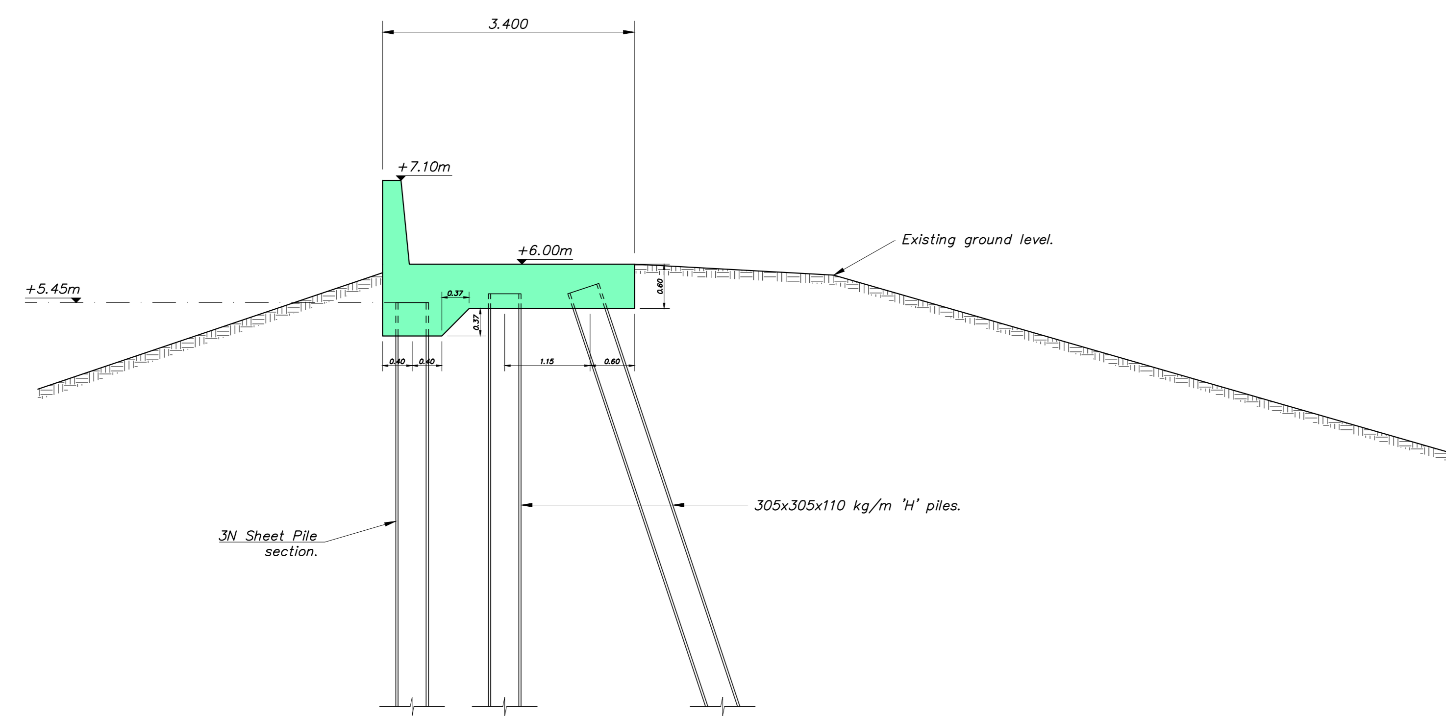
Typical Section Existing Wall Type 2 - Structural Wall 1:50
