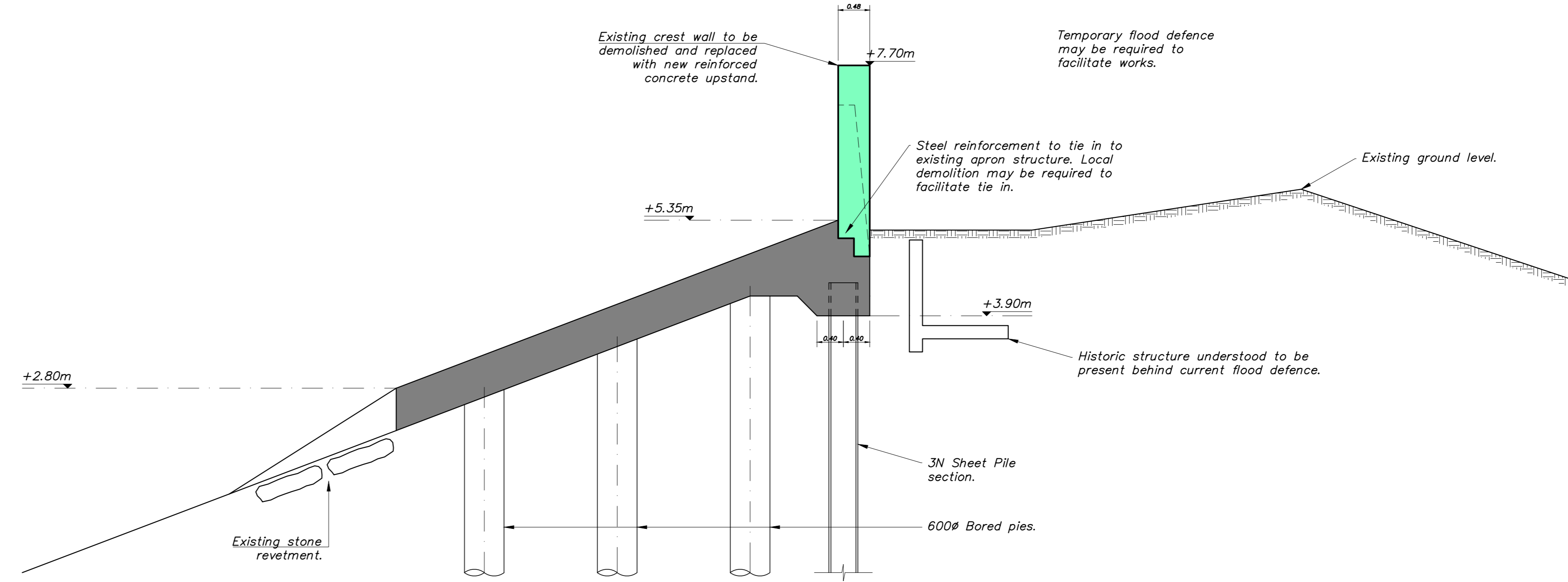
Typical Section. Existing Wall Type 3 - Reinforced Concrete Apron on CFA Piles Option B - New Crest Wall 1:50
